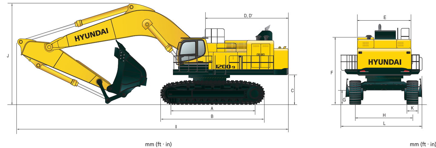
DIMENSIONS R1200-9
