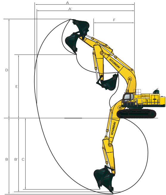
WORKING RANGE R1200-9
